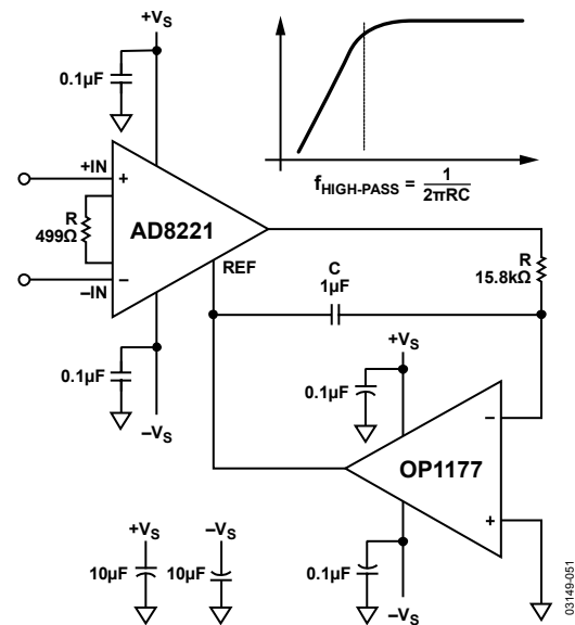
Figure 52. AC-Coupled Circuit
