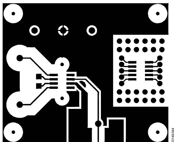
Figure 45. Top Layer of the AD8221-EVAL
