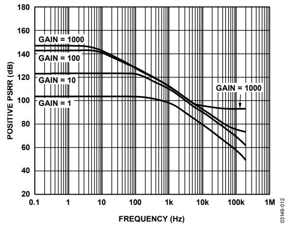
Figure 13. Positive PSRR vs. Frequency, RTI ( G = 1 to 1000)
