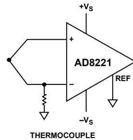
THERMOCOUPLE
