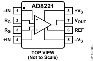
Figure 3. Pin Configuration
