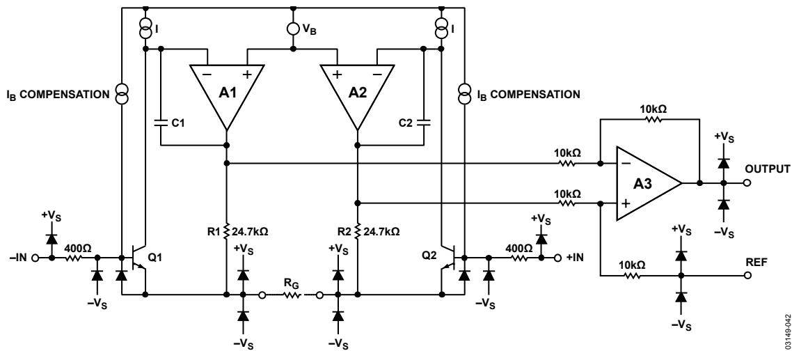
Figure 43. Simplified Schematic
