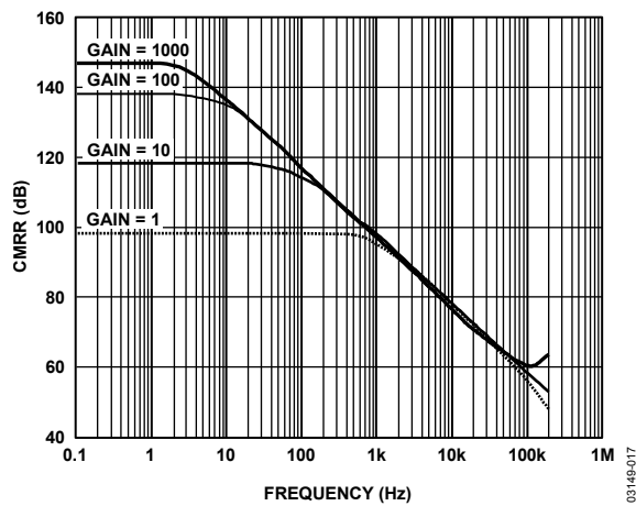
Figure 18. CMRR vs. Frequency, RTI, 1 kΩ Source Imbalance
