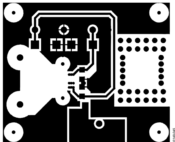
Figure 46. Bottom Layer of the AD8221-EVAL
