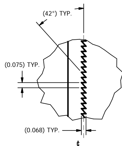
DETAIL G APERTURE RIGHT EDGE (POND OF MIRRORS OMITTED FOR CLARITY) SCALE 60 : 1
