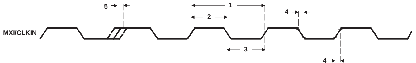
Figure 6-15. M24XI Timing
