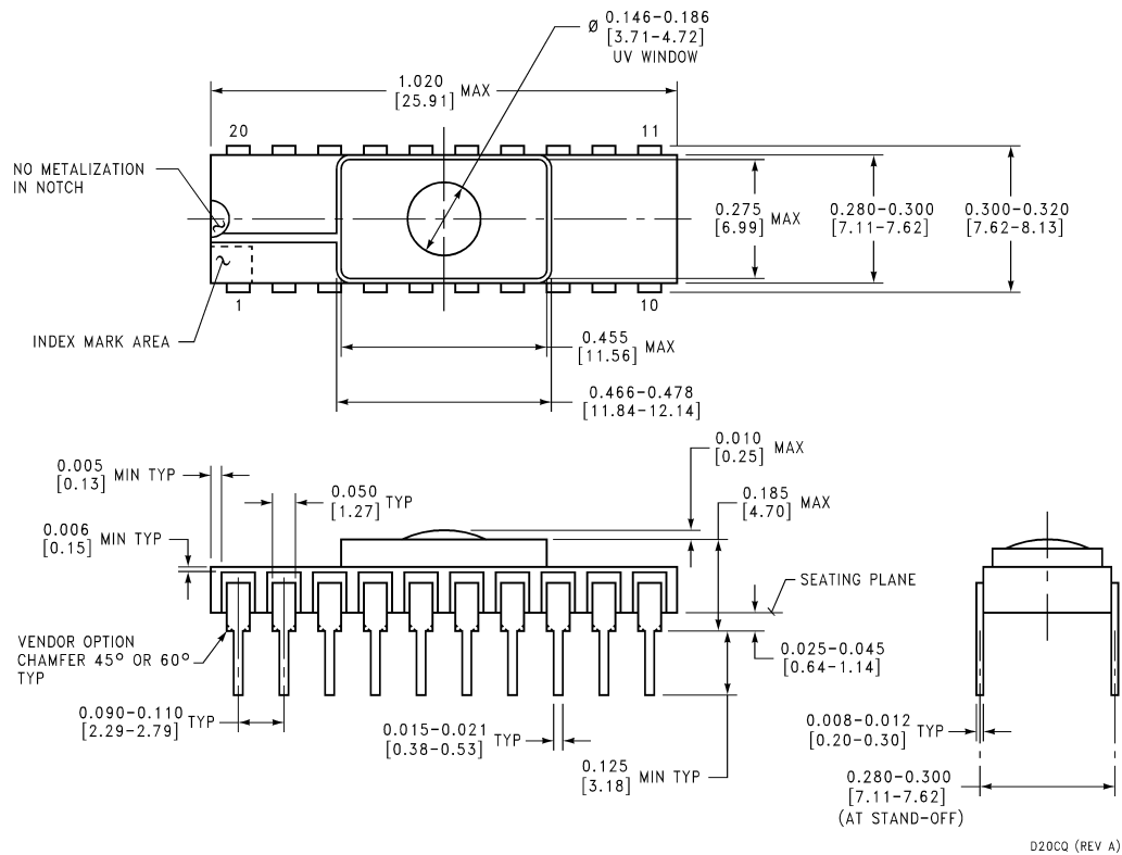
20-Lead Hermetic Dual-In-Line Package, EPROM (D) Order Number COP8SAC720Q3 NS Package Number D20CQ
