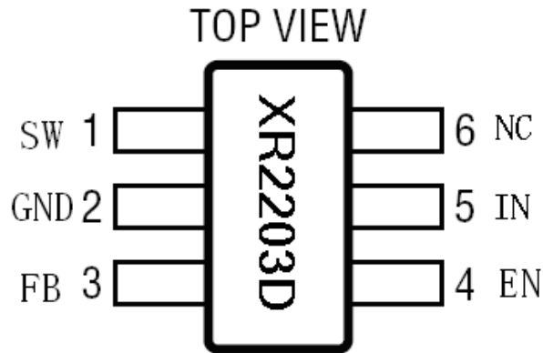
Figure 2 PIN Configuration
