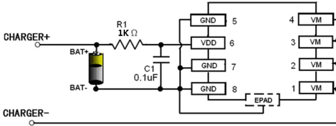
Fig 6 XB8089G in a Typical Battery Protection Circuit
