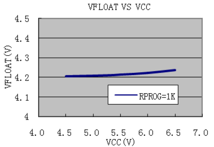
BATTERY CHARGER CURVE
