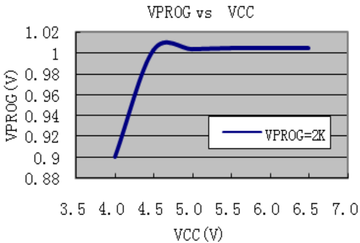
BATTERY CHARGER CURVE
