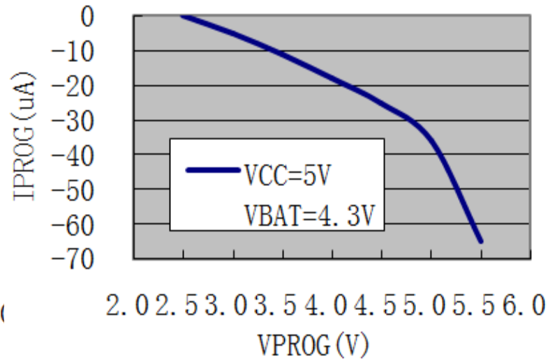
PROG CLAMP CURRENT VS VPROG
