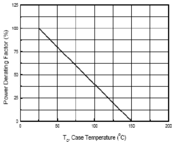
Fig.5 Power Derating
