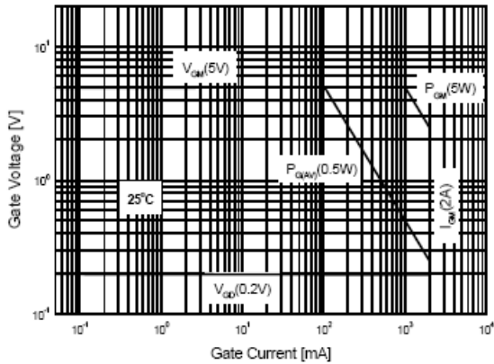
Fig.1 Gate Characteristics
