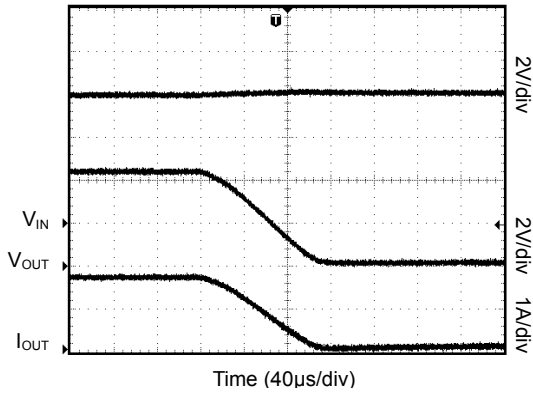
Soft-Stop during OCP Event
