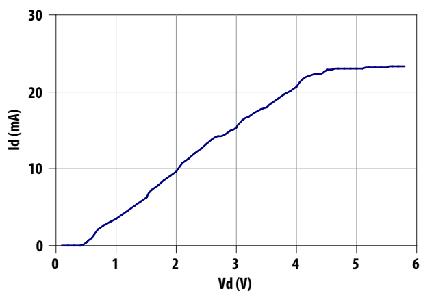
Figure 8. Total Current at V_c = 5\text{V} [1]
